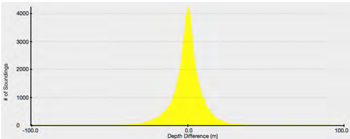
Histogram of sounding-depth differences from cross-line check of Line 281 and dipline 232 (smooth bathymetry). Kongsberg Maritime EM122.
