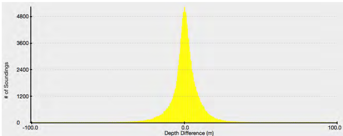
Histogram of sounding-depth differences from cross-line check of Line 330 and dipline 230 (smooth bathymetry). Kongsberg Maritime EM122.
