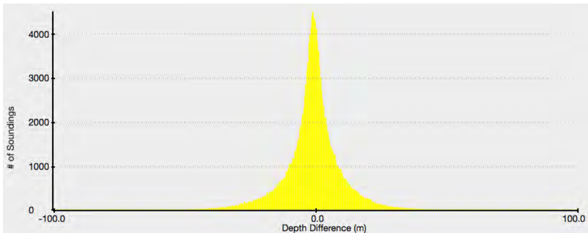
Histogram of sounding-depth differences from cross-line check of Line 297 and dipline 231 (smooth bathymetry). Kongsberg Maritime EM122.
